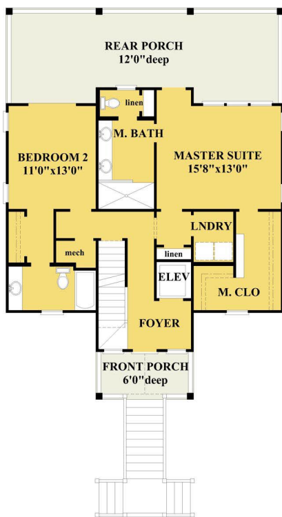
FIRST FLOOR PLAN 1009 HEATED SQUARE FEET
