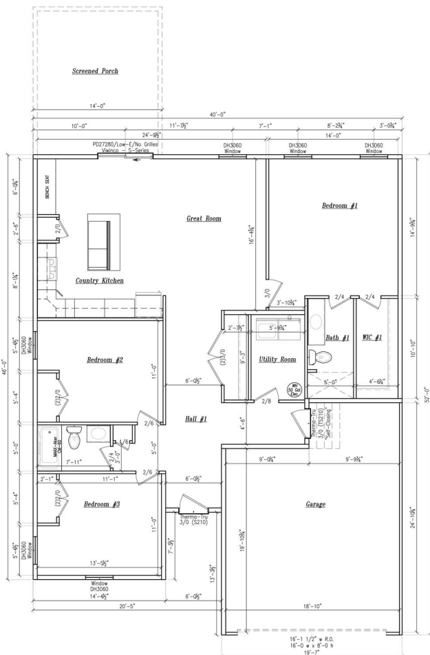
First Floor Plan - New Layout SCALE 3/16" = 1'-0"
